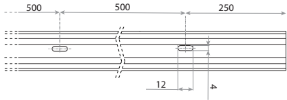
Rail detail
