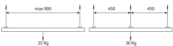
Maximale belasting
